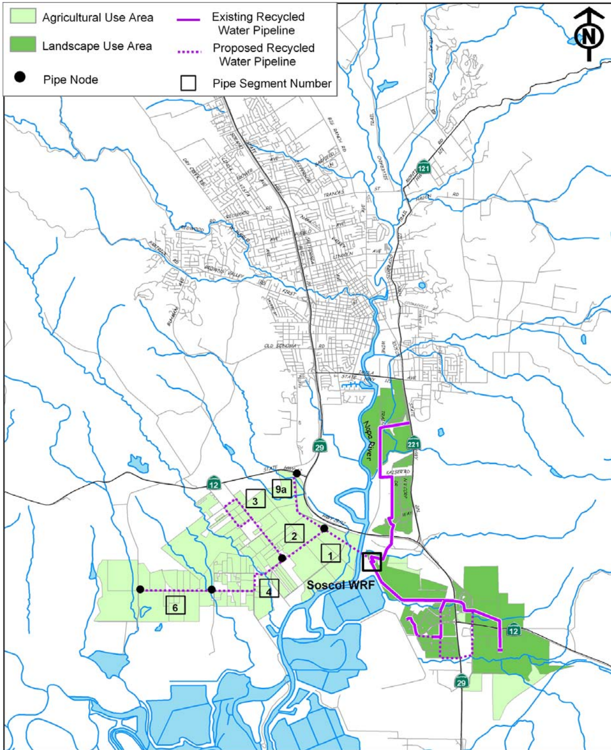
Figure 2-13 Strategy No. 6: Deliver Recycled Water to Carneros Area
